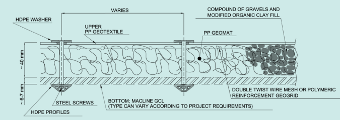
Remedial Sealing Mattress (RSM)
