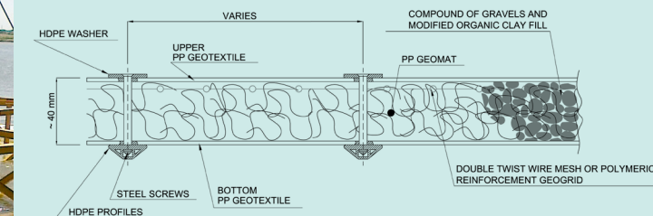
Remedial Filtering Mattress (RFM)
