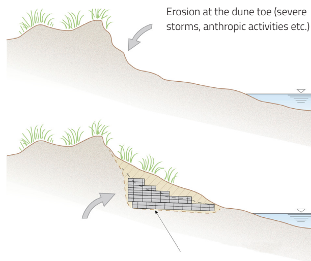
Dune core reconstruction from Gabions, Reno Mattresses®, MacTubes®, MacBags®, MacGrids® as appropriate
