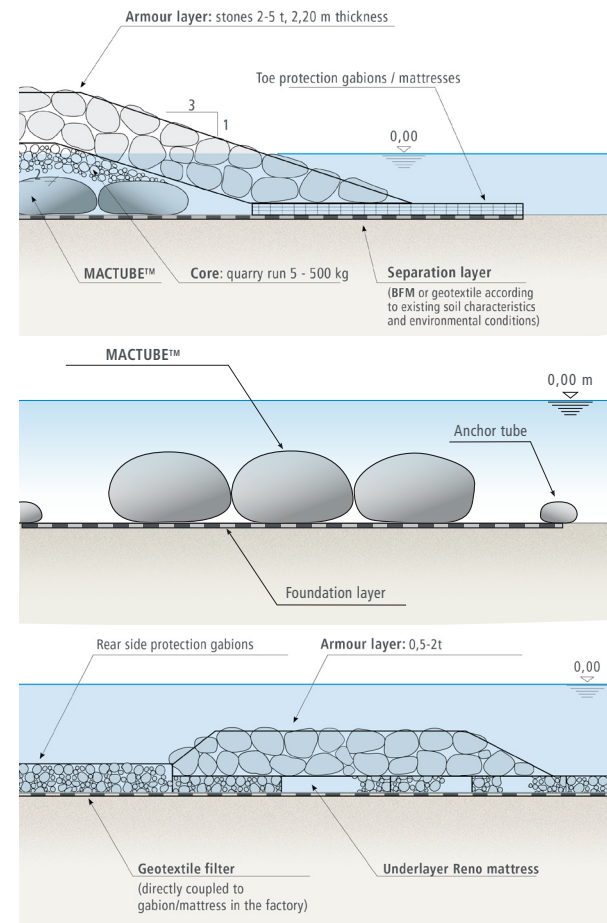
Typical cross-section
