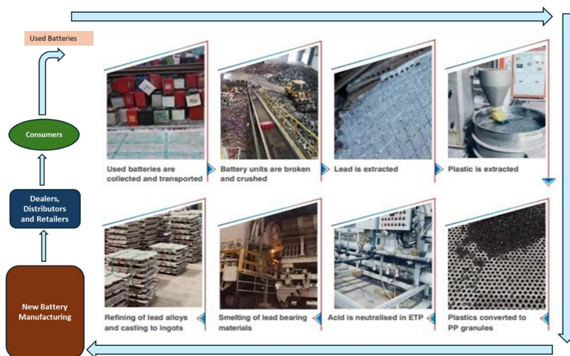
Exhibit 26: Lead Acid Battery Recycling Process
