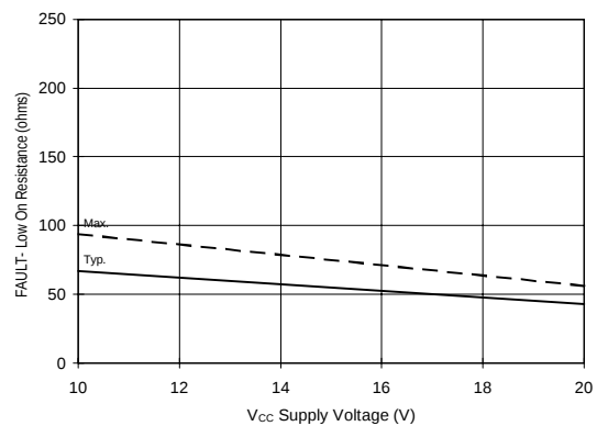
Figure 37B. \overline{FAULT} Low On Resistance vs. Voltage
