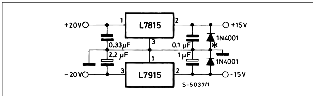
Figure 4: Split Power Supply ( \pm 15\text{V}/1\text{A} )
