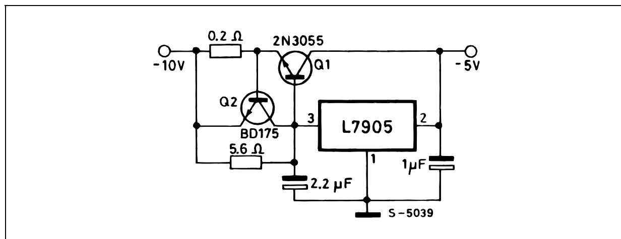
Figure 6: High Current Negative Regulator ( -5\text{V}/4\text{A} with 5A current limiting)
