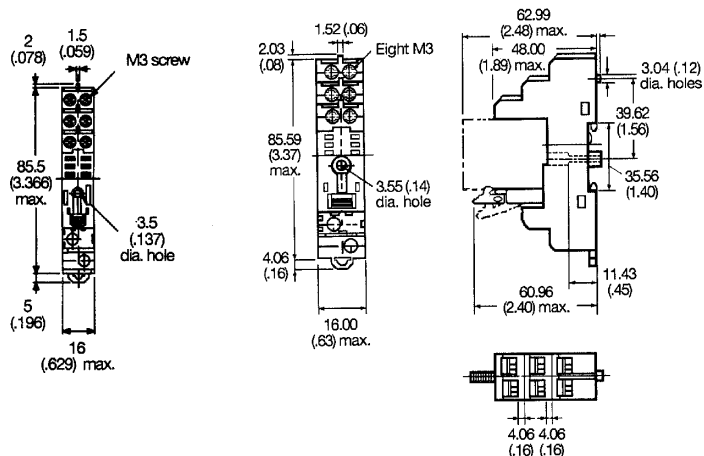
Terminal arrangement
