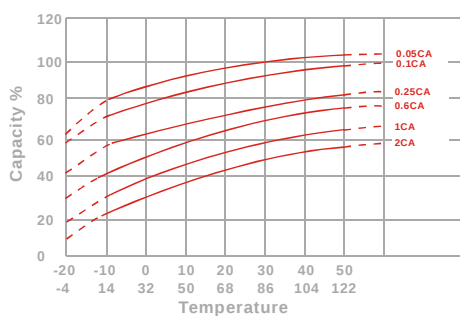
Effect of Temperature on Capacity 25 (77 °C)
