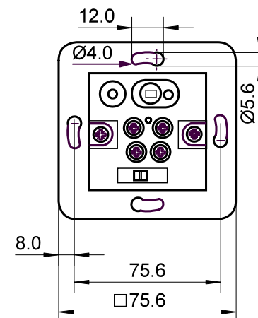
Montageansicht Mounting view
