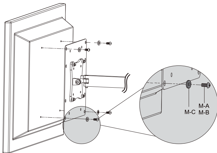
Fig.8: Mounting the flat screen
