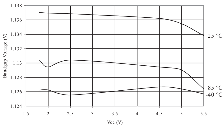
Figure 33-34. Calibrated Bandgap Voltage vs. V_{CC}
