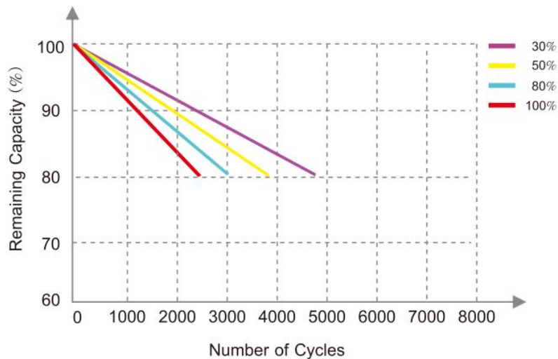
Different DOD Discharge Cycle Life Curve(1C)
