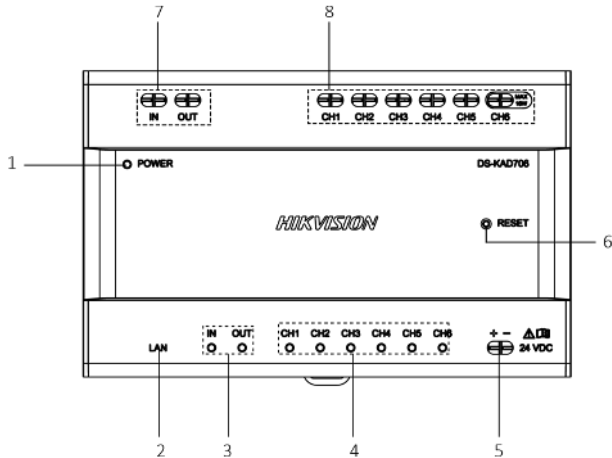
Figure 1-1 Video/Audio Distributor Appearance
