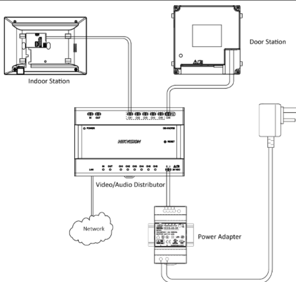
Figure 2-1 Wiring Description
