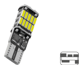
ASX3026 - T10 W5W 300lm - 12/24v - 2,5w - 35mm - 26 SMD LEDS Canbus
