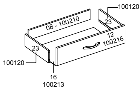
GAVETA DRAWER CAJÓN
