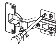
Ajuste tornillos frontales Front screws adjustment
