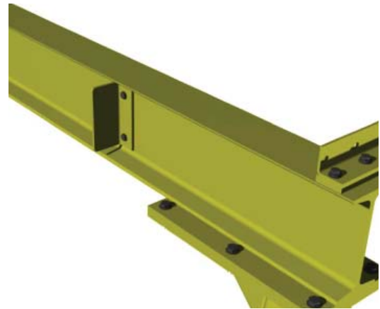
AS INSTALLED
