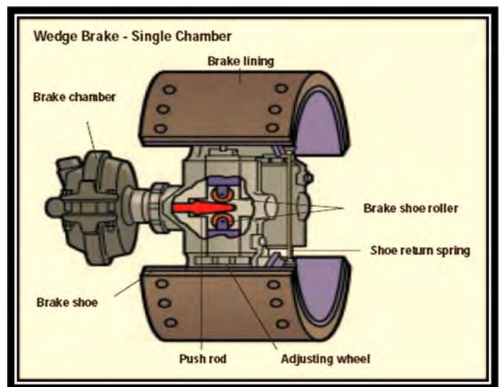
Figure 5.2a Wedge Brake
