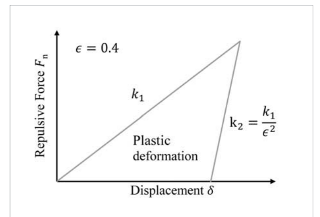
Fig. 2: Relationship between particle \delta overlap and Force F_n for restitution coefficient \epsilon=0.4 (from [3])
