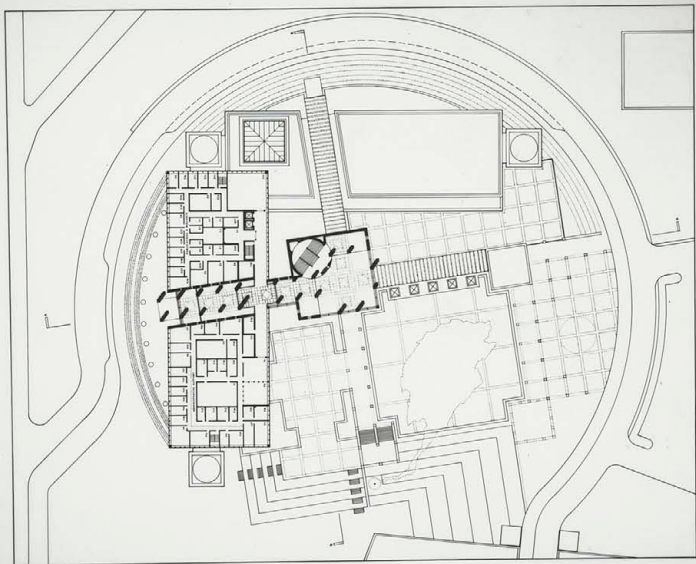
ADMINISTRATIVE LEVEL
