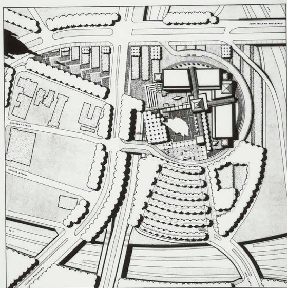
SITE PLAN
