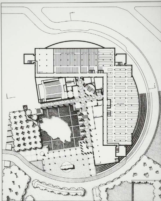
PARK LEVEL
