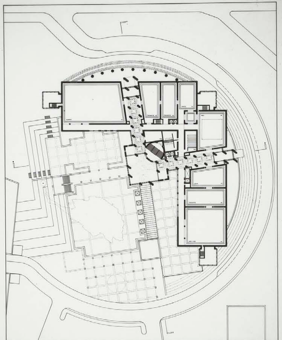
GALLERY LEVEL
