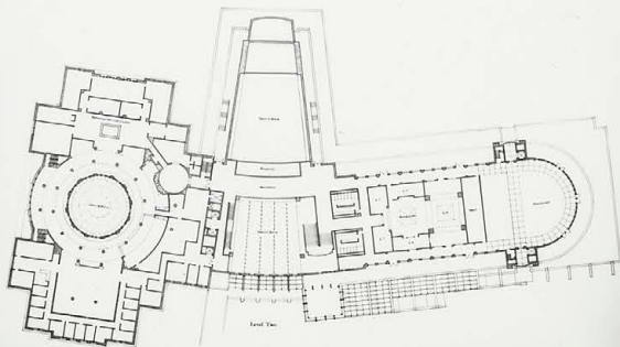
Level Two
