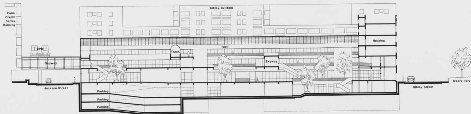
ST. PAUL LOWERTOWN BLOCK 40 DEVELOPMENT EAST-WEST SECTION
