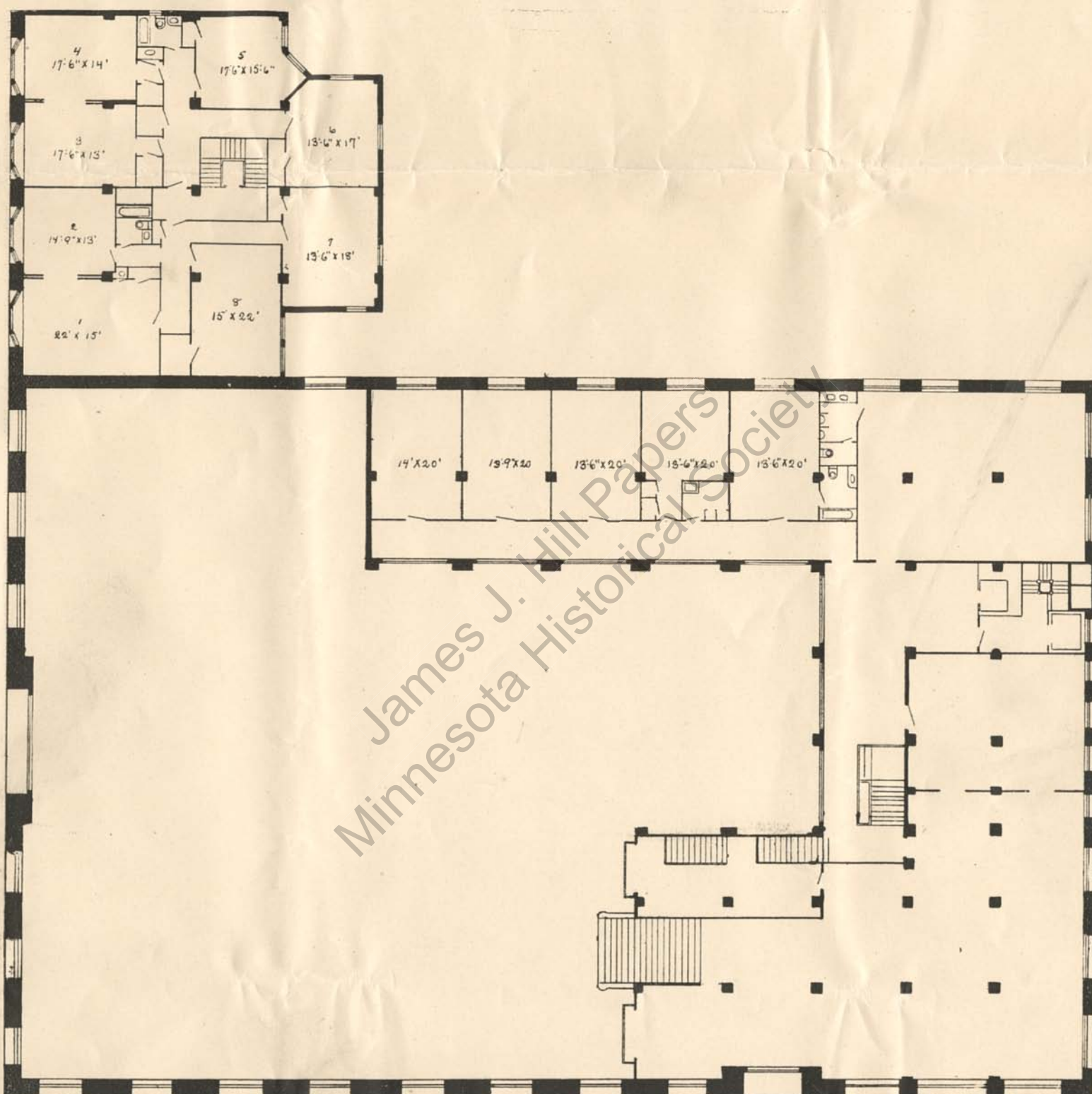
MEZZANINE FLOOR
