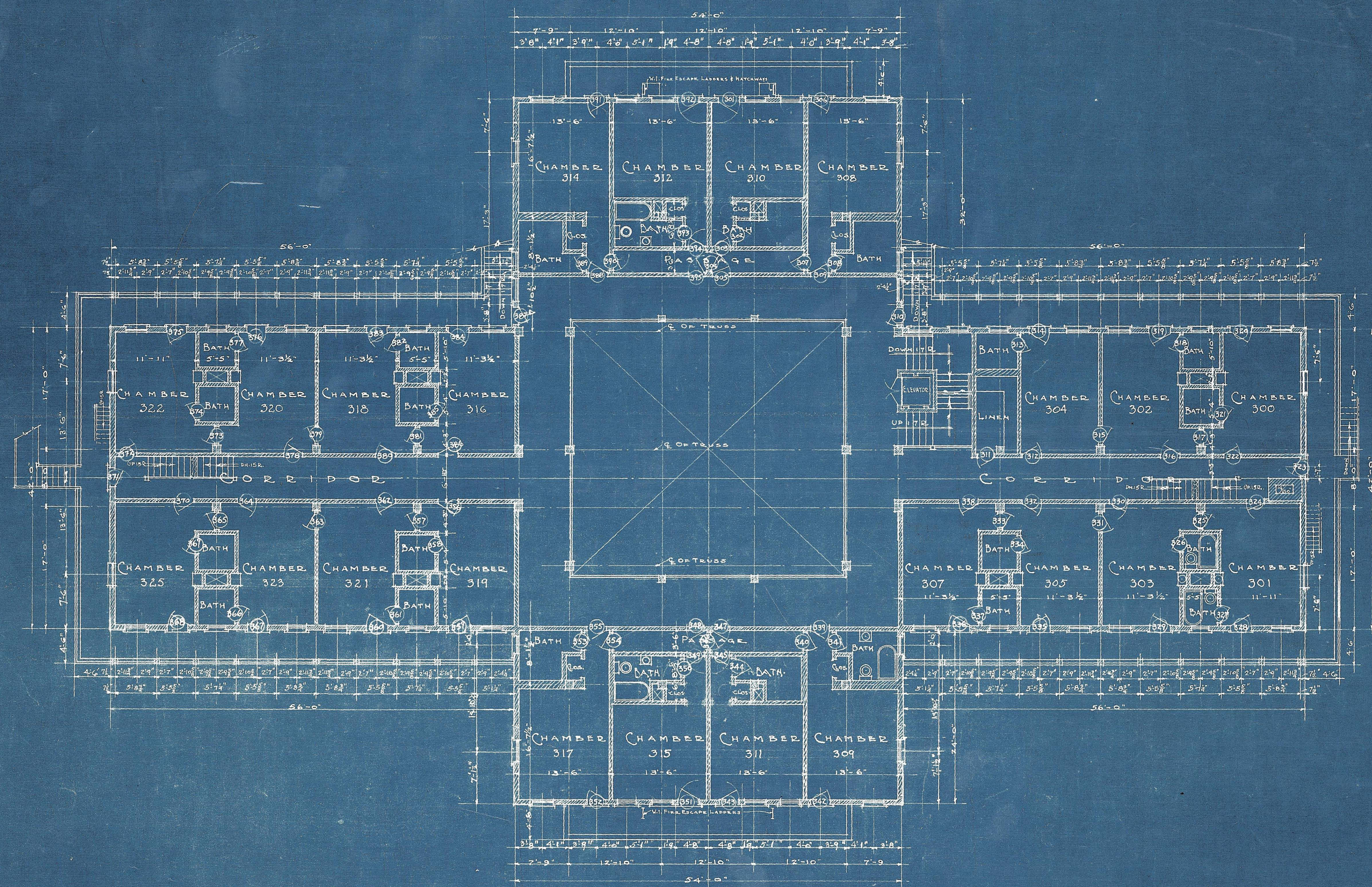
THIRD FLOOR PLAN SCALE 1/8"=1'-0"
