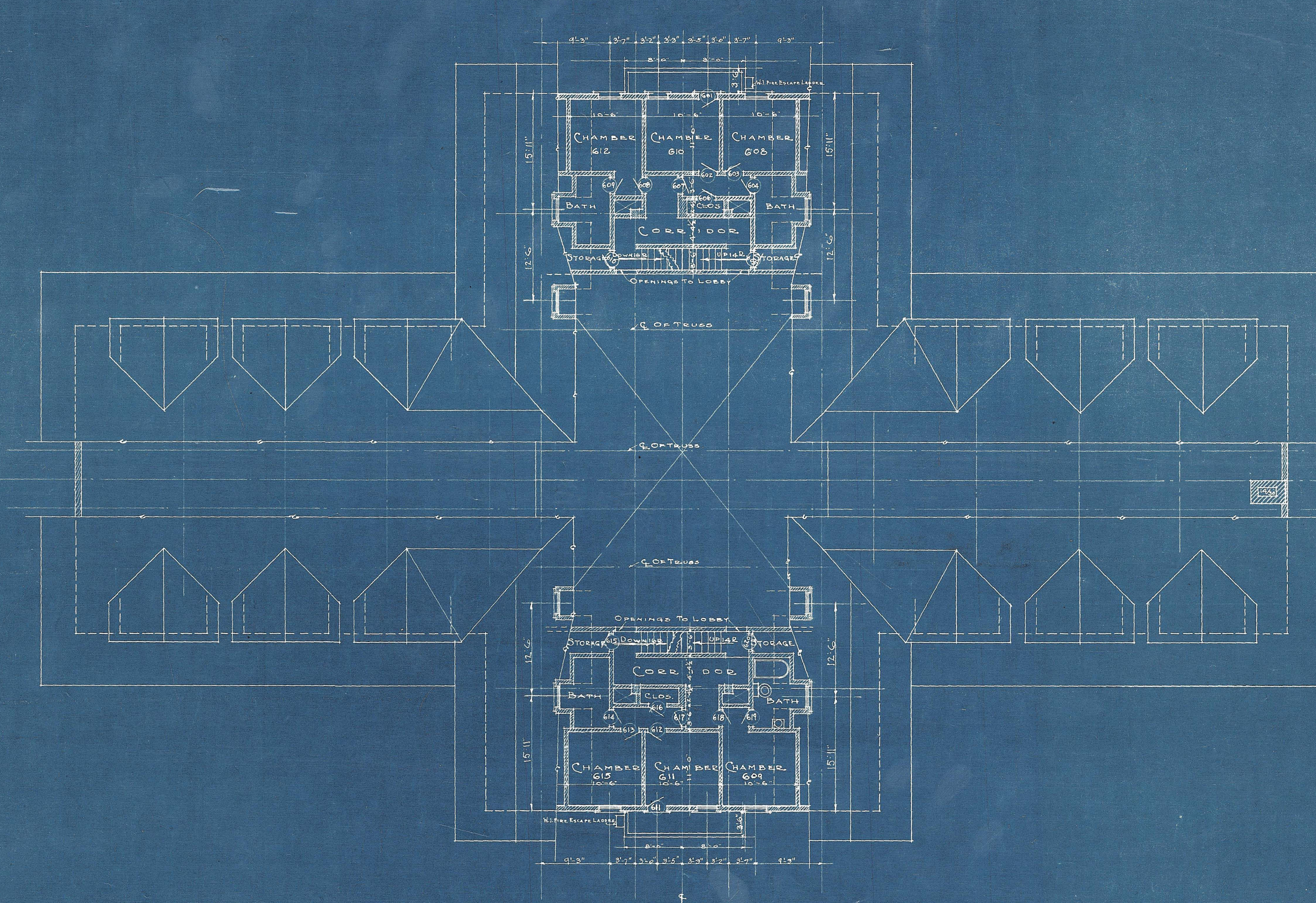
SIXTH FLOOR PLAN SCALE 1/8"=1'-0"
