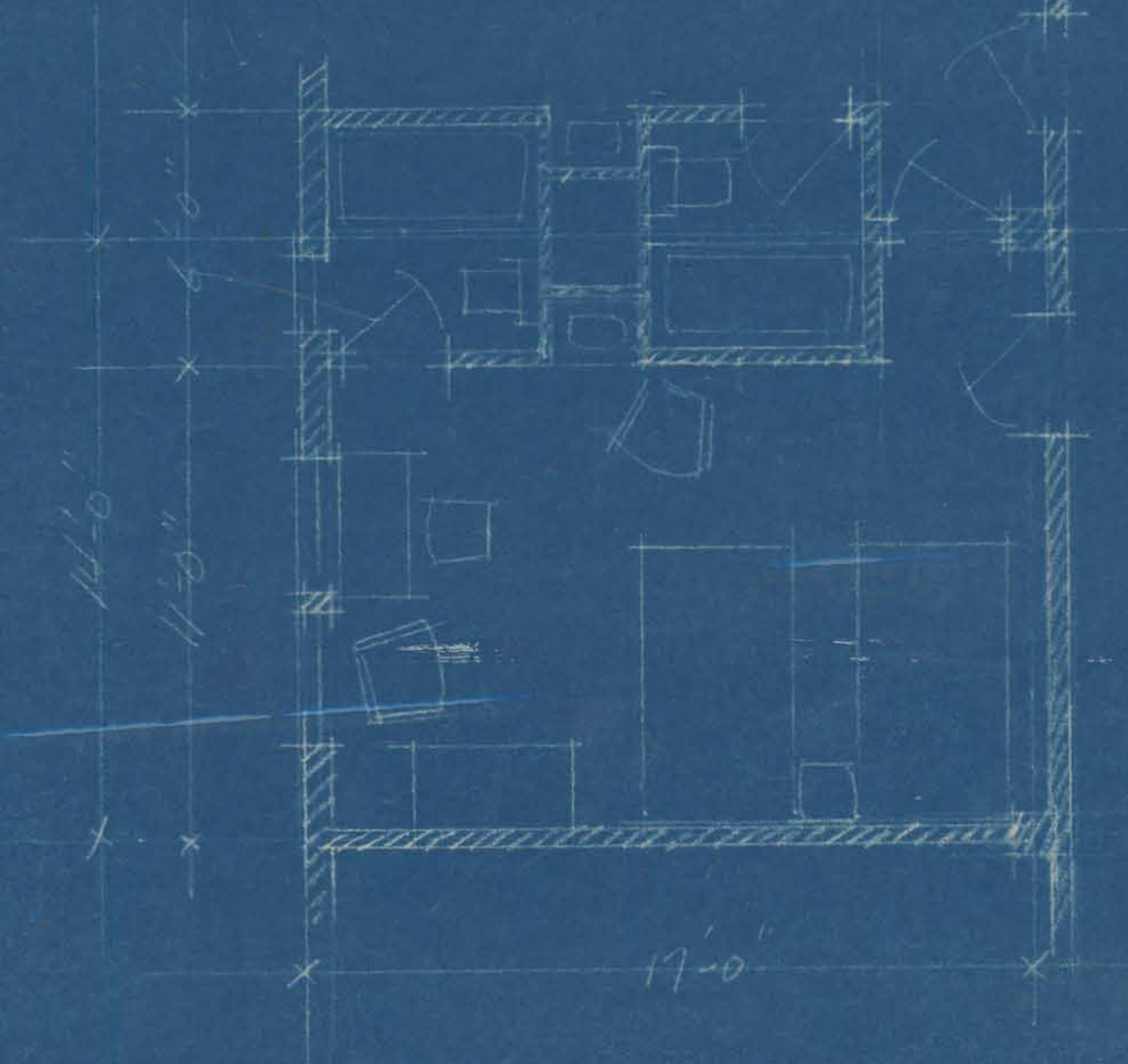
TYPICAL BED ROOM AT 1/4" SCALE
