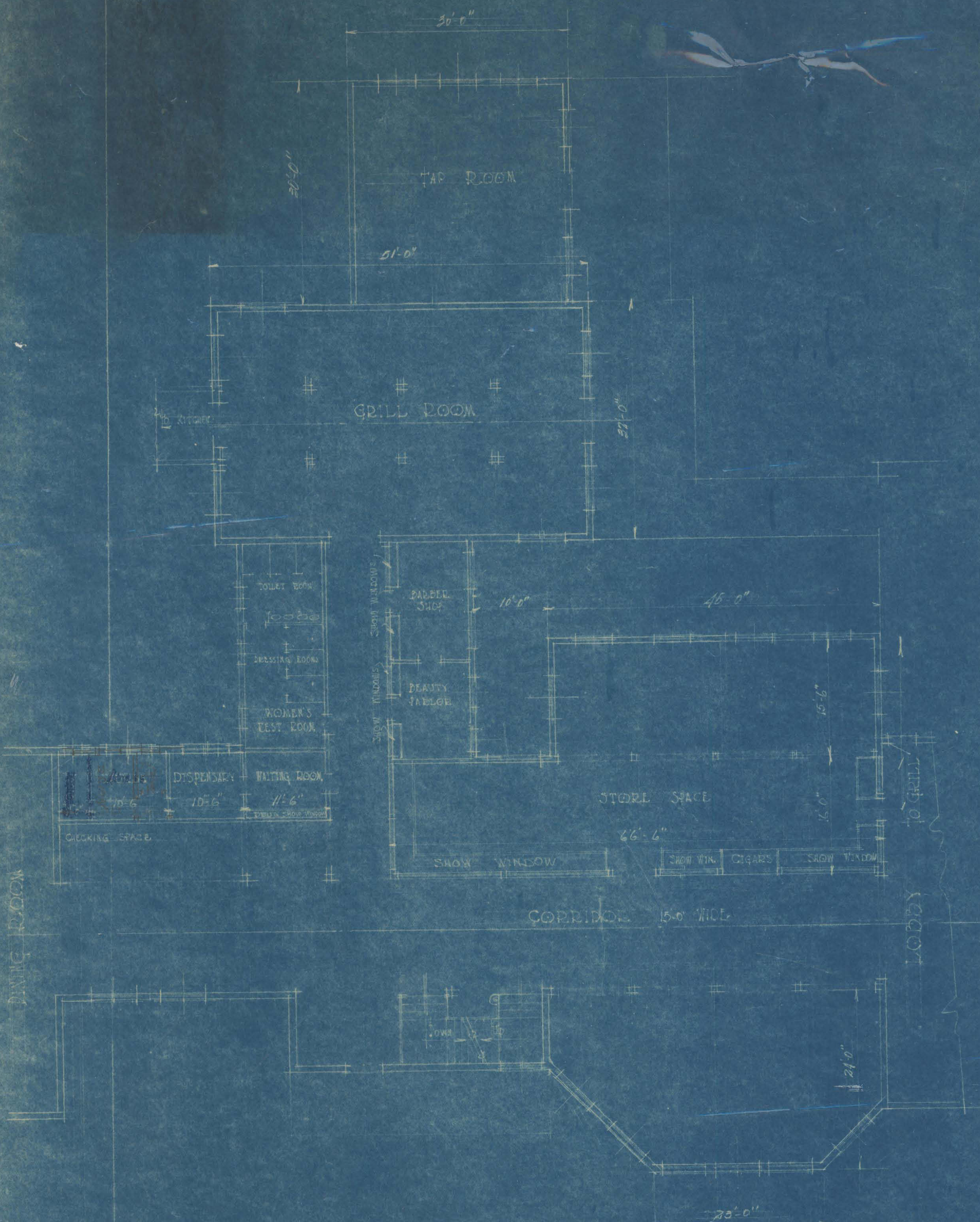
FIRST FLOOR PLAN - STORE & GRILL UNIT
