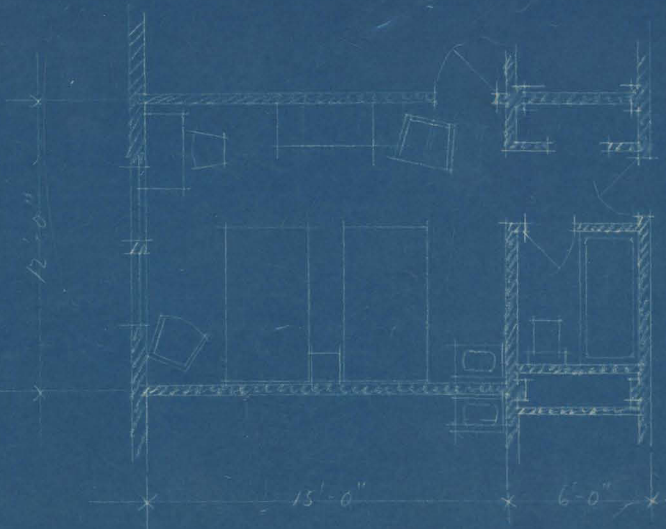
TYPICAL BEDROOM AT 1/4 IN. SCALE
