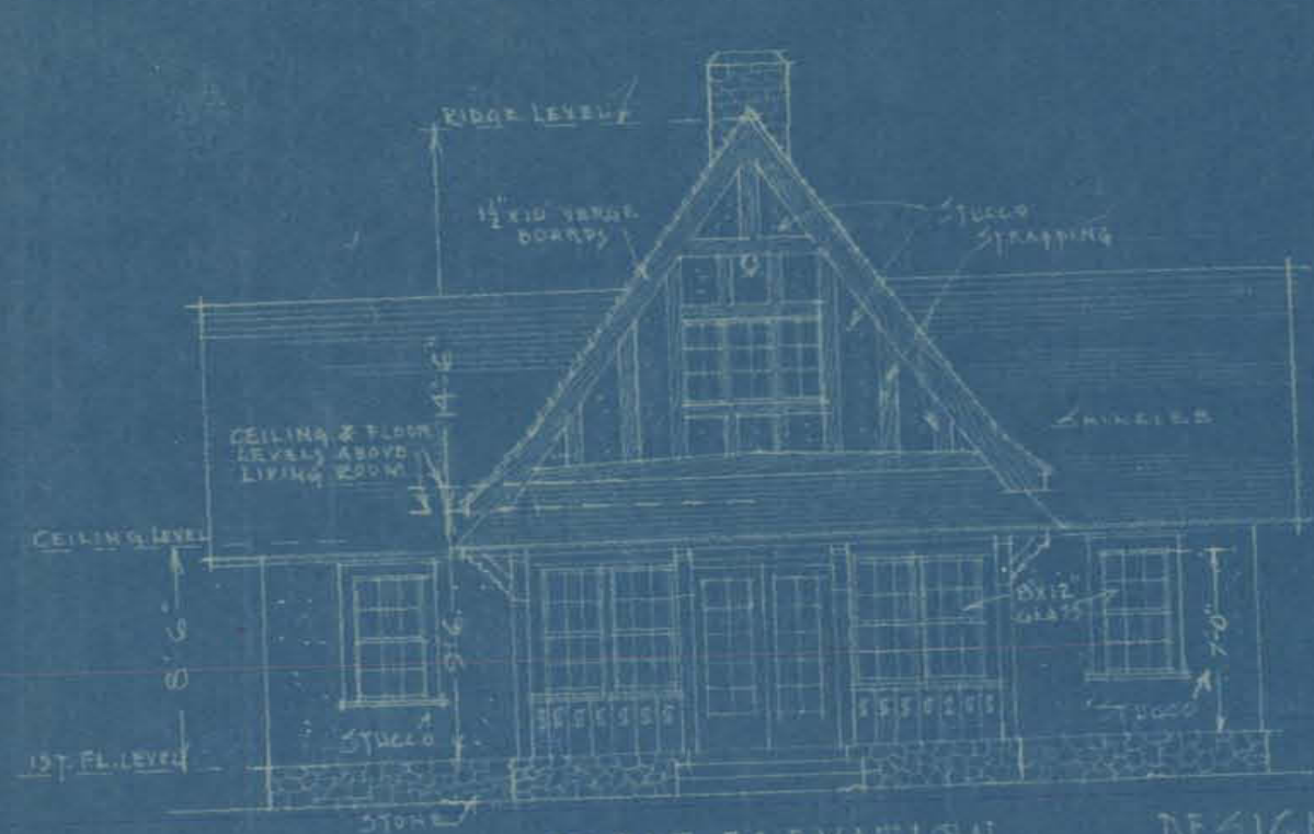
FRONT ELEVATION DESIGN A
