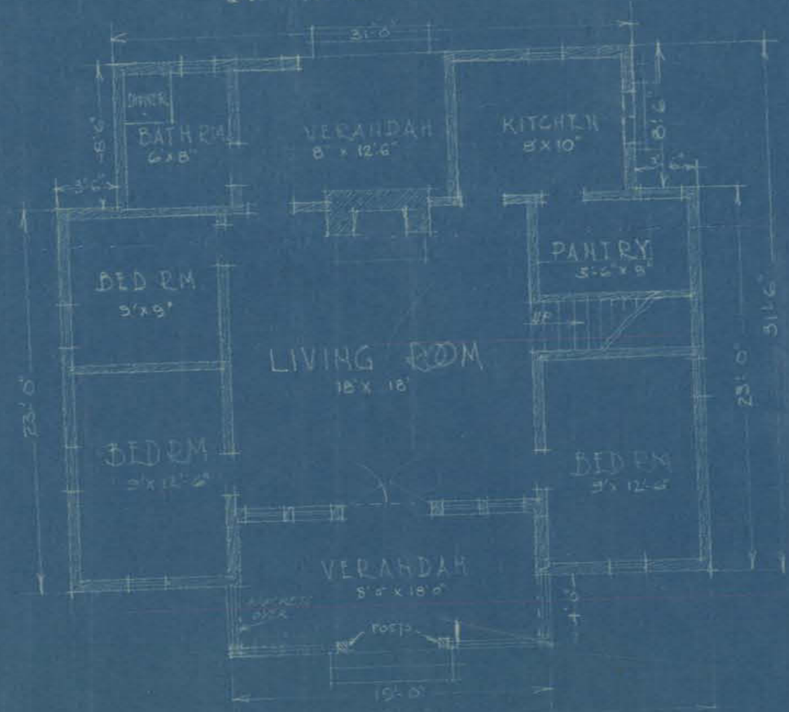
FIRST FLOOR PLAN DESIGN B
