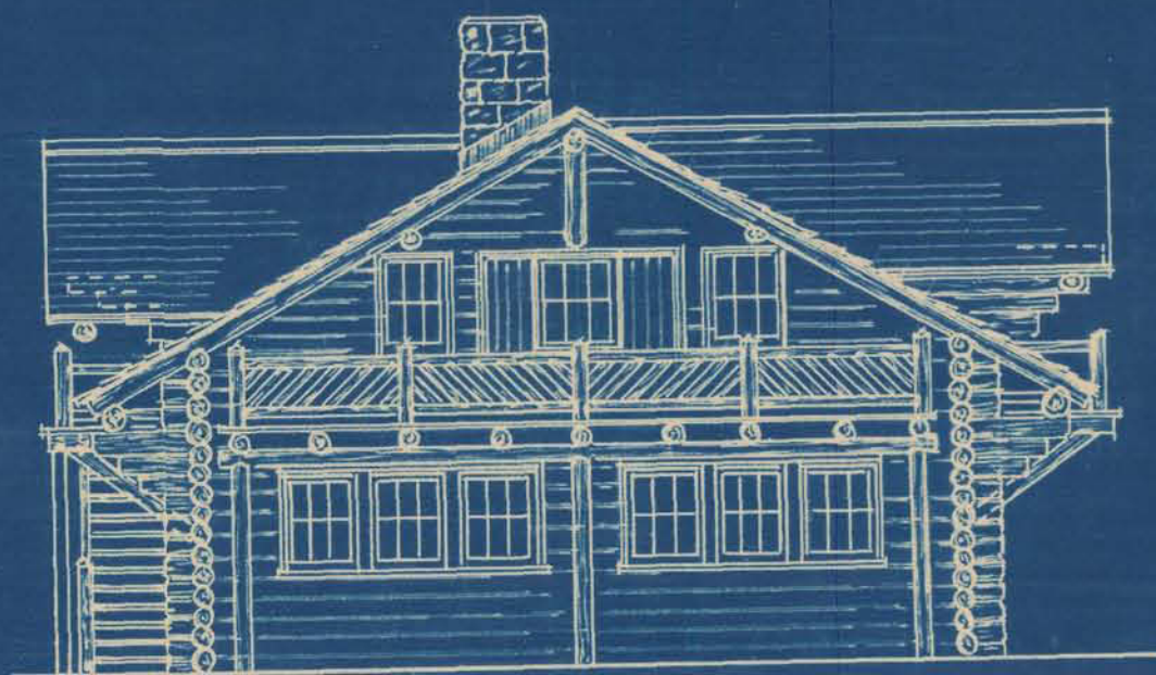
SIDE ELEVATION SCALE \frac{1}{8}" = 1'-0"
