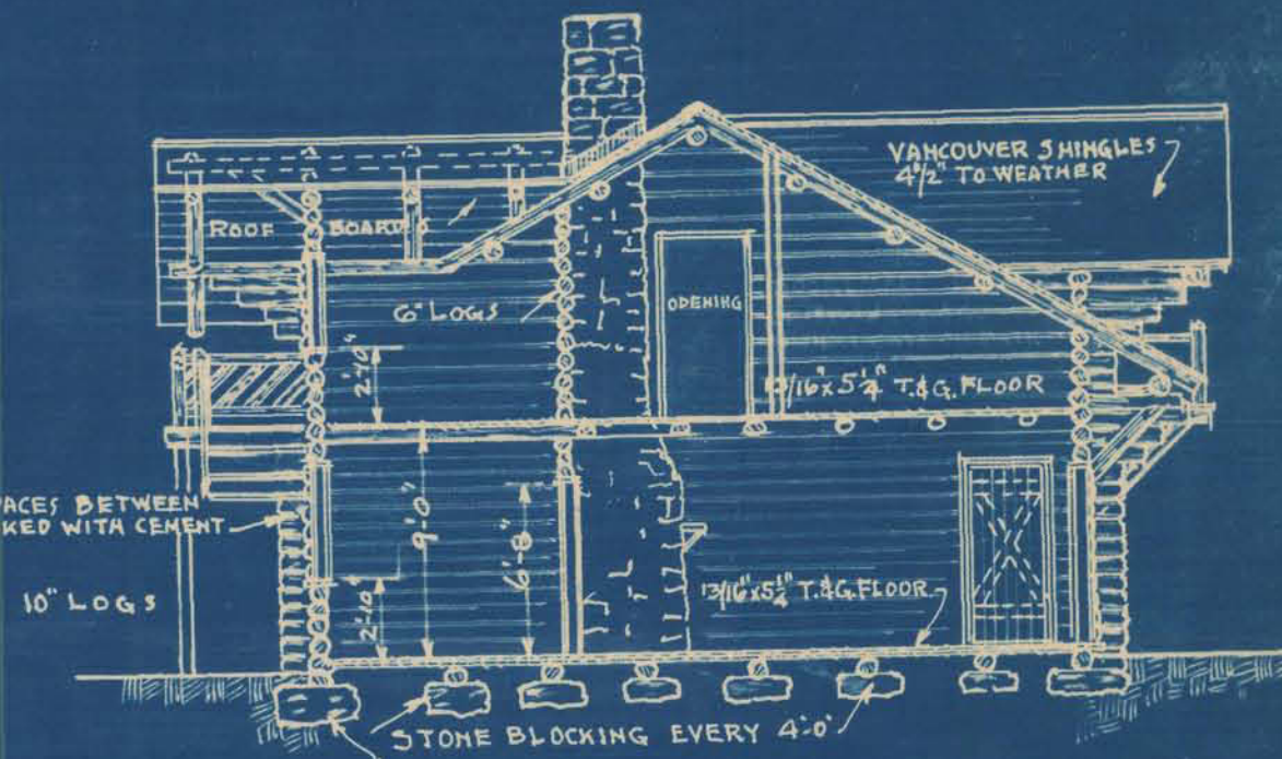
CROSS SECTION. SCALE \frac{1}{4}" = 1'-0"
