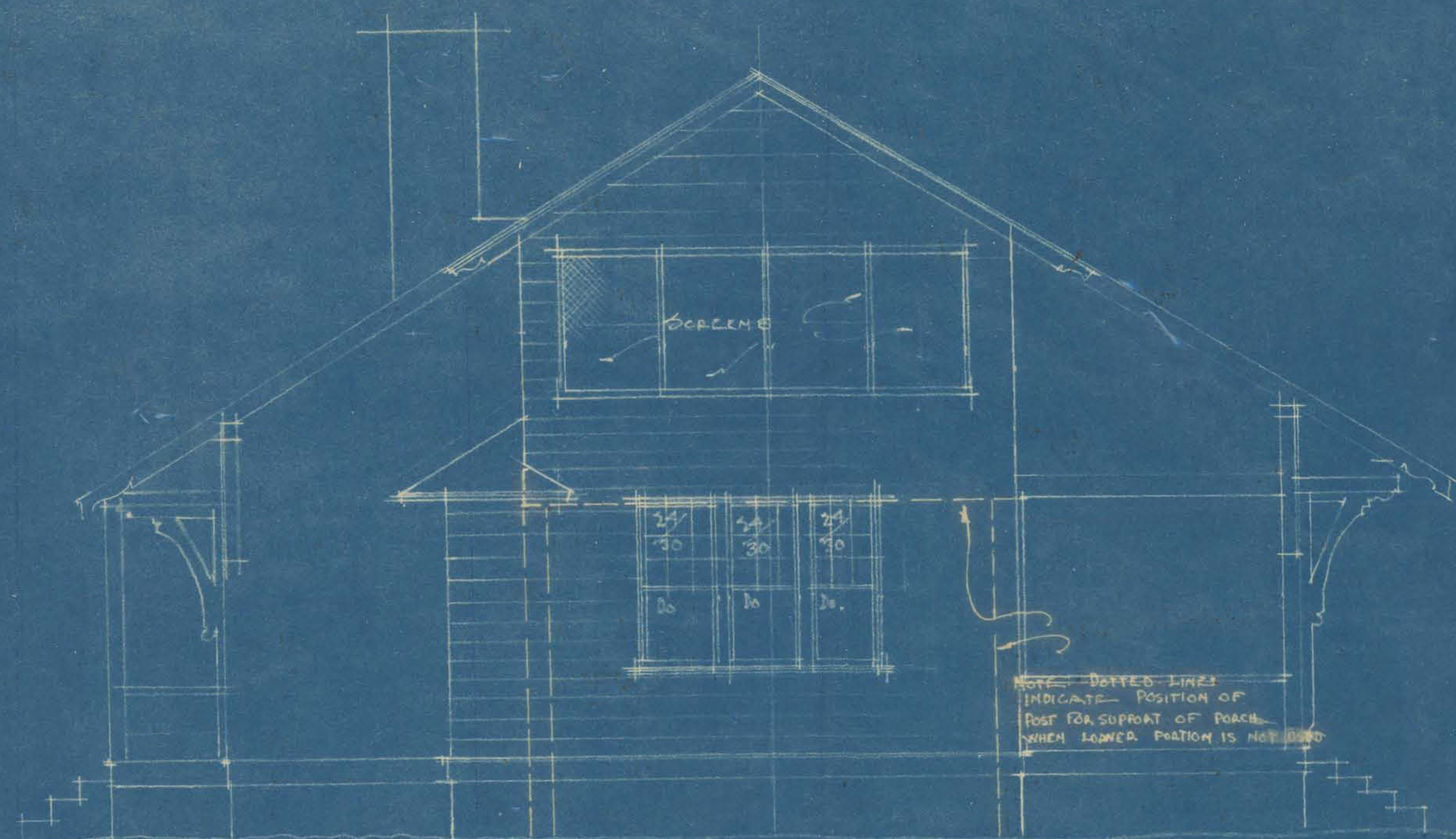
SIDE ELEVATION.
