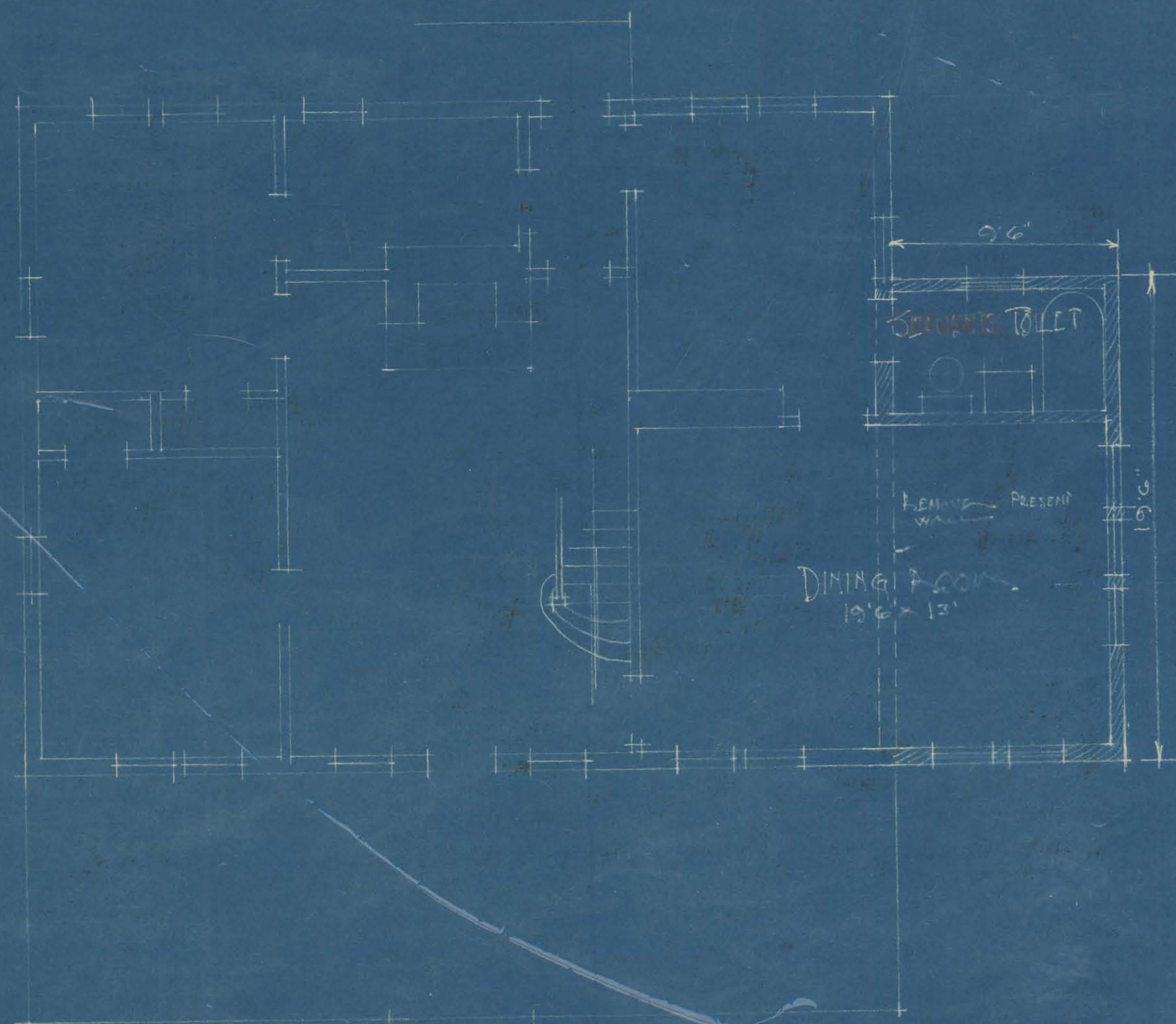
FIRST FLOOR 1/4" = 1'0"
