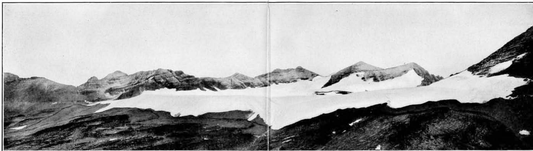
FIG. 12.—SPERRY GLACIER FROM LITTLE MATTERHORN, GUNSIGHT MOUNTAIN IN BACKGROUND. Photograph by W. C. Alden.
