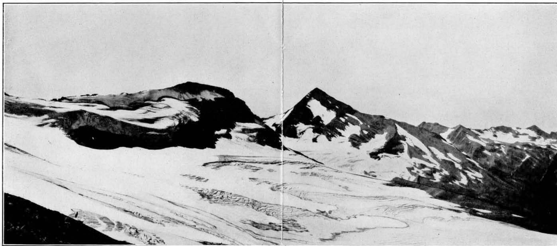
FIG. 13.—BLACKFEET GLACIER, EASTERN PART, BLACKFOOT MOUNTAIN AND JACKSON MOUNTAIN IN BACKGROUND. Photograph by W. C. Alden.
