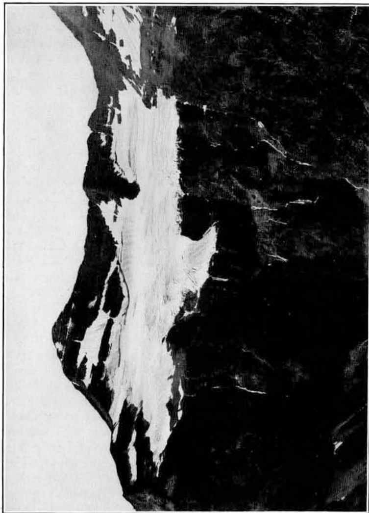
FIG. 23.—RAINBOW GLACIER, RAINBOW PEAK IN BACKGROUND. Photograph by M. R. Campbell.
