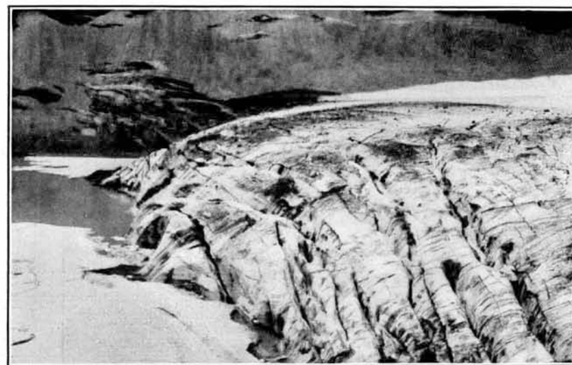
FIG. 15.—FRONT OF GLACIER AT ICEBERG LAKE. Photograph by W. C. Alden.
