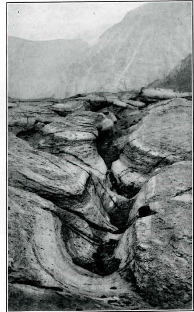
FIG. 6.—GLACIATED GROOVE NEAR FRONT OF SPERRY GLACIER.
