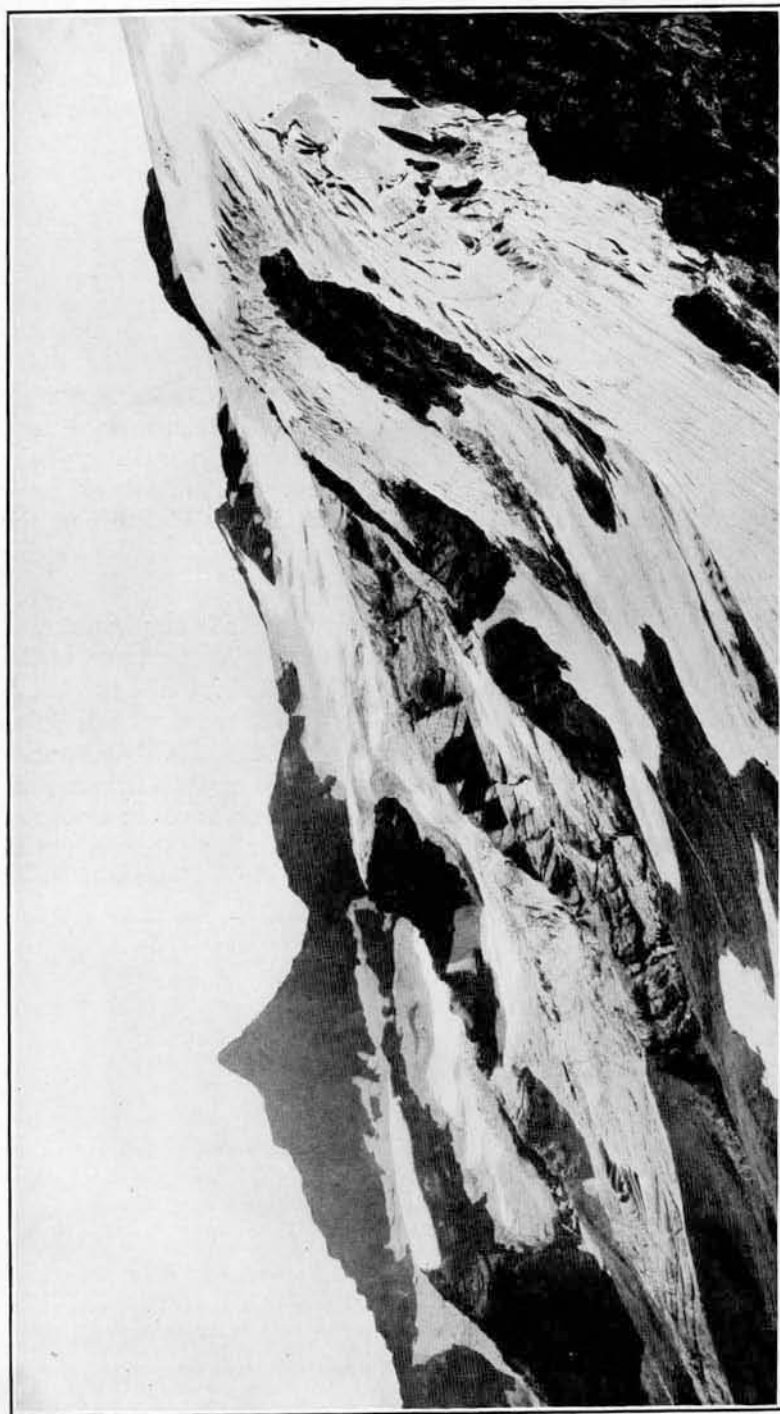
FIG. 2.—HARRISON GLACIER, SHOWING THE CASCADING FRONTAL LOBES. Photograph by W. C. Alden.
