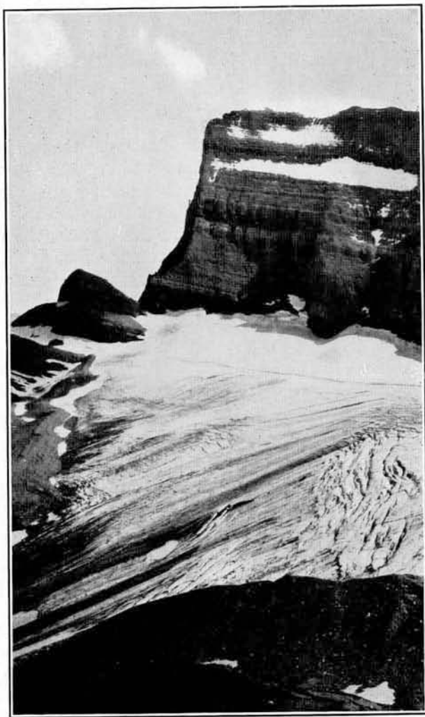
FIG. 7.—GOULD MOUNTAIN AND GRINNELL GLACIER. Morainal ridge at left and in foreground. Photograph by T. W. Stanton.
