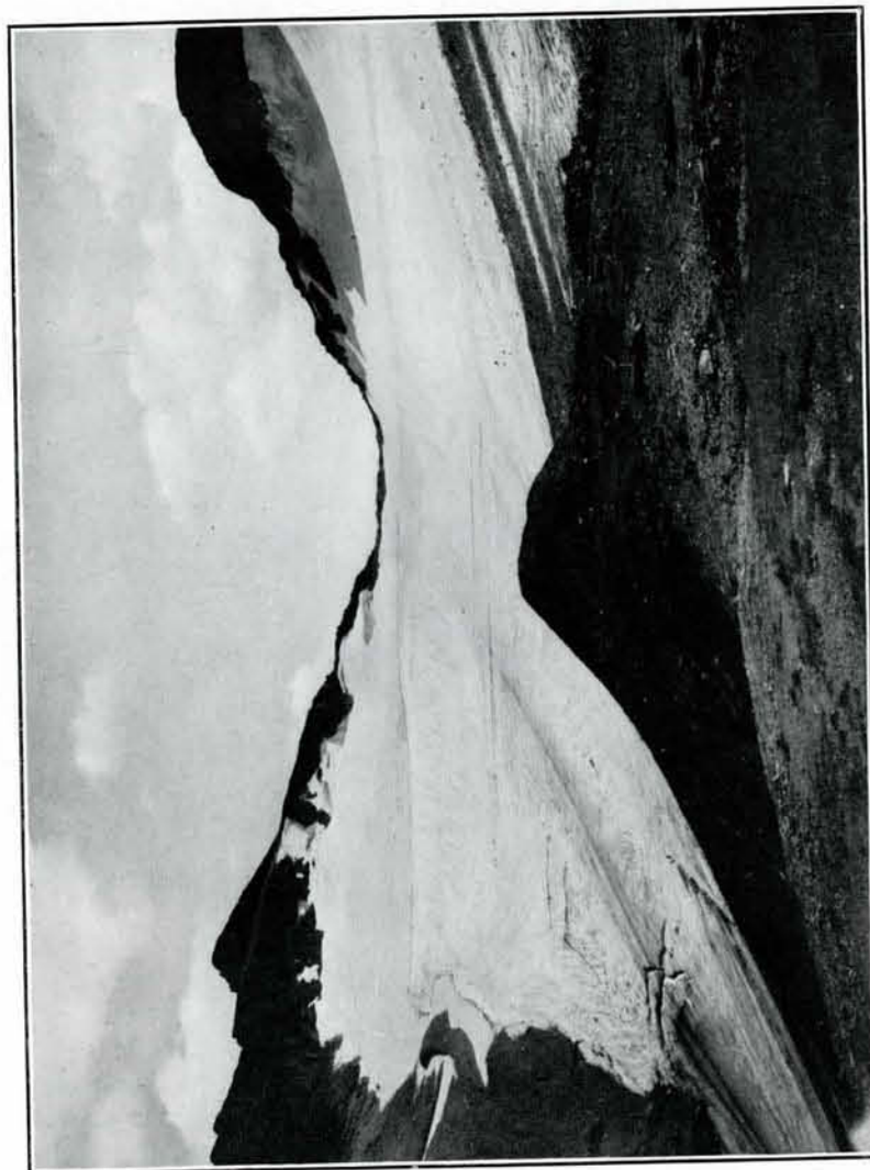
FIG. 20.—CHANNEY GLACIER. Terminal moraine in foreground, medial moraine at right.
