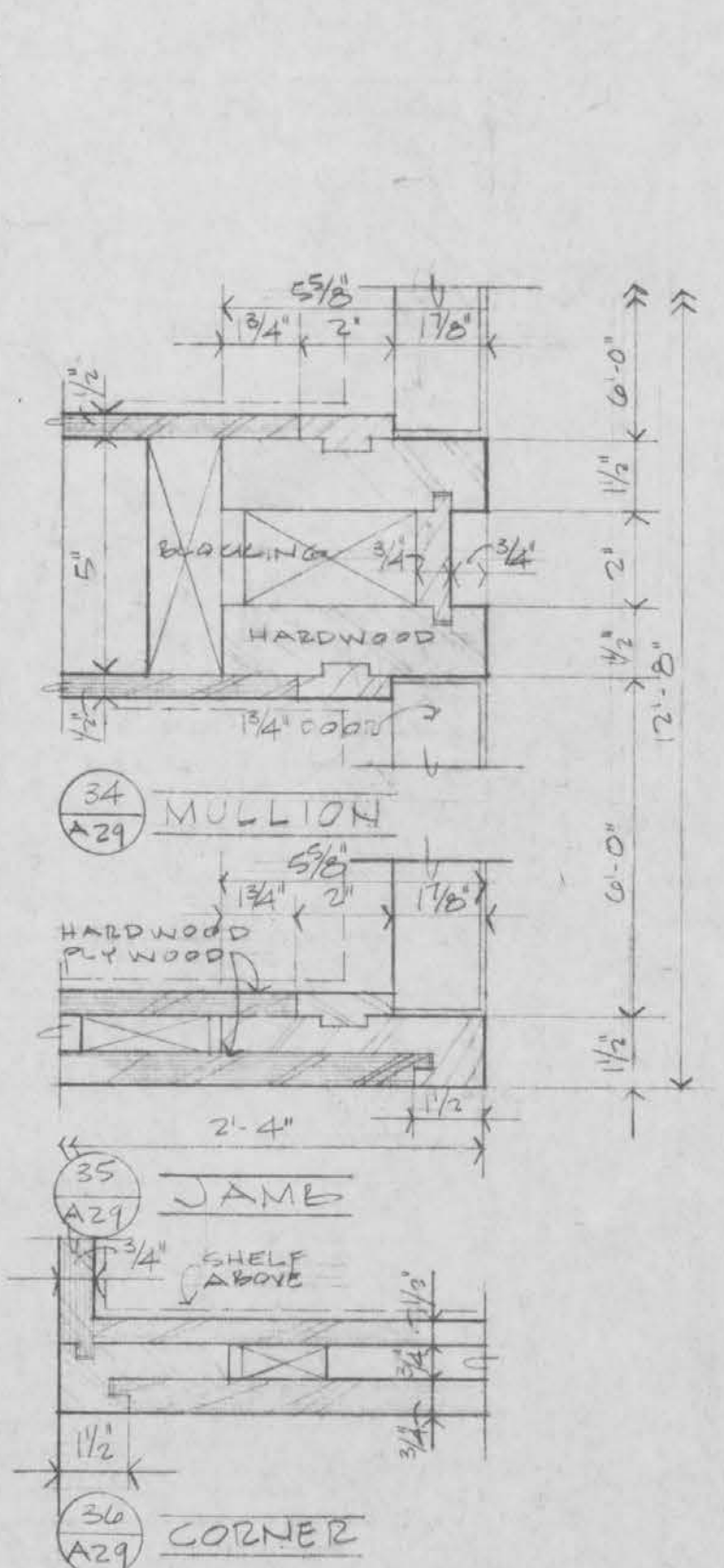
CAB. DETS. RM. 12-210 SCALE: 3" = 1'-0"
