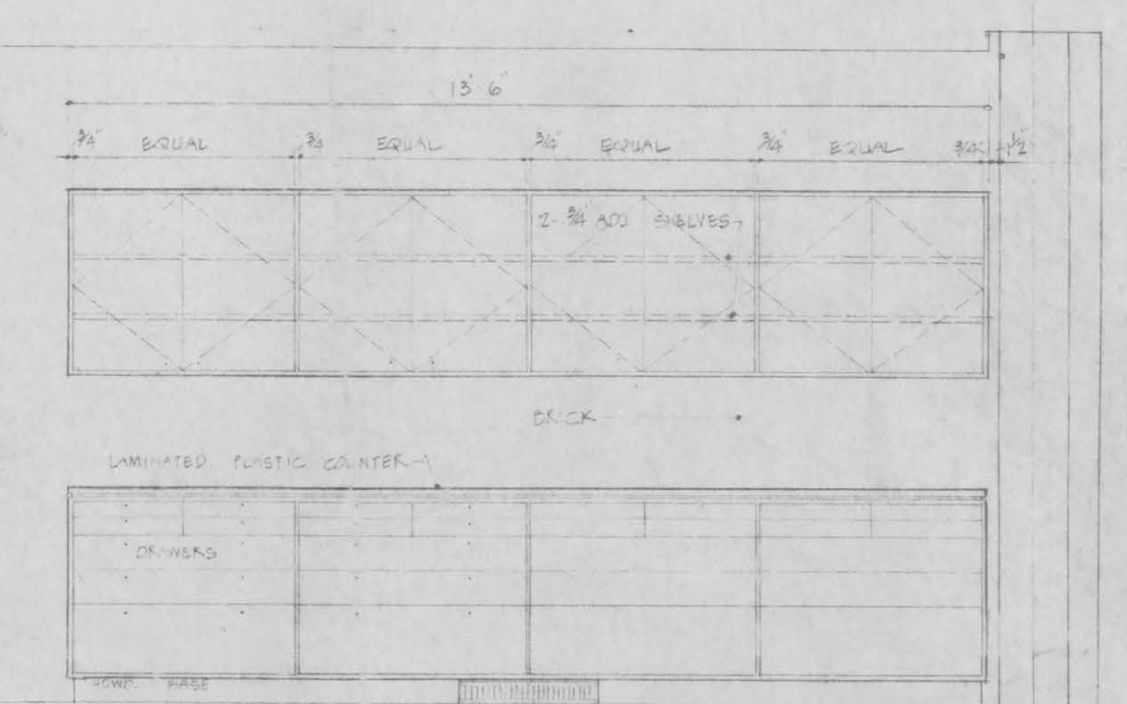
24' x 4' R.A. G.E. L.L.E. BASE BY GEN. CONTR. ELEVATION OF WORK COUNTER R-244
