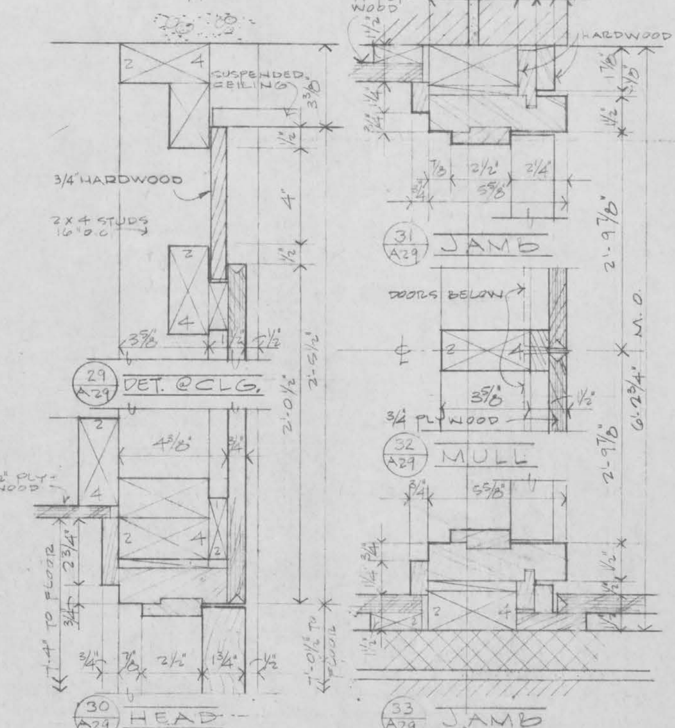
16 (29) MILLWORK DETAILS @ CLOSET R-212 SCALE: 3" = 1'-0"
