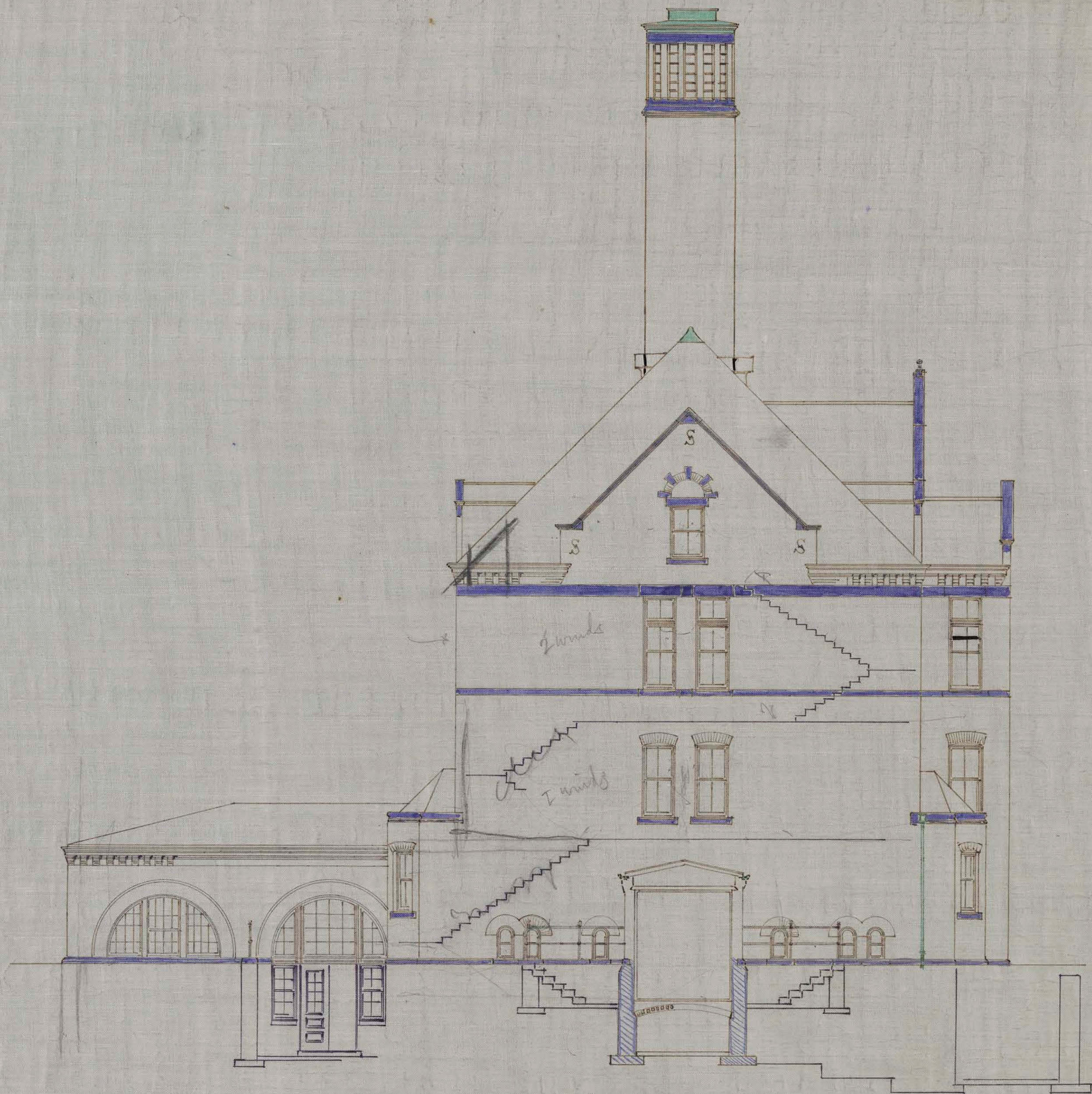
^ SOUTH ELEVATION ^
