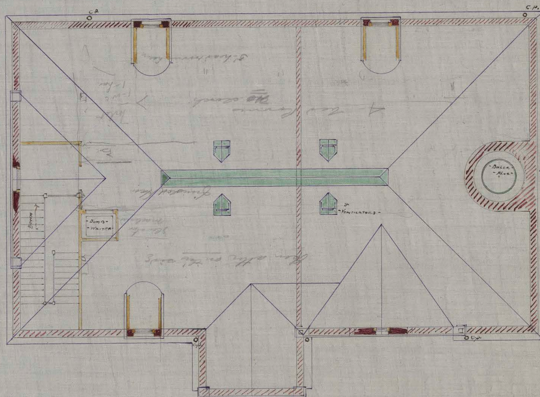
ATTIC PLAN
