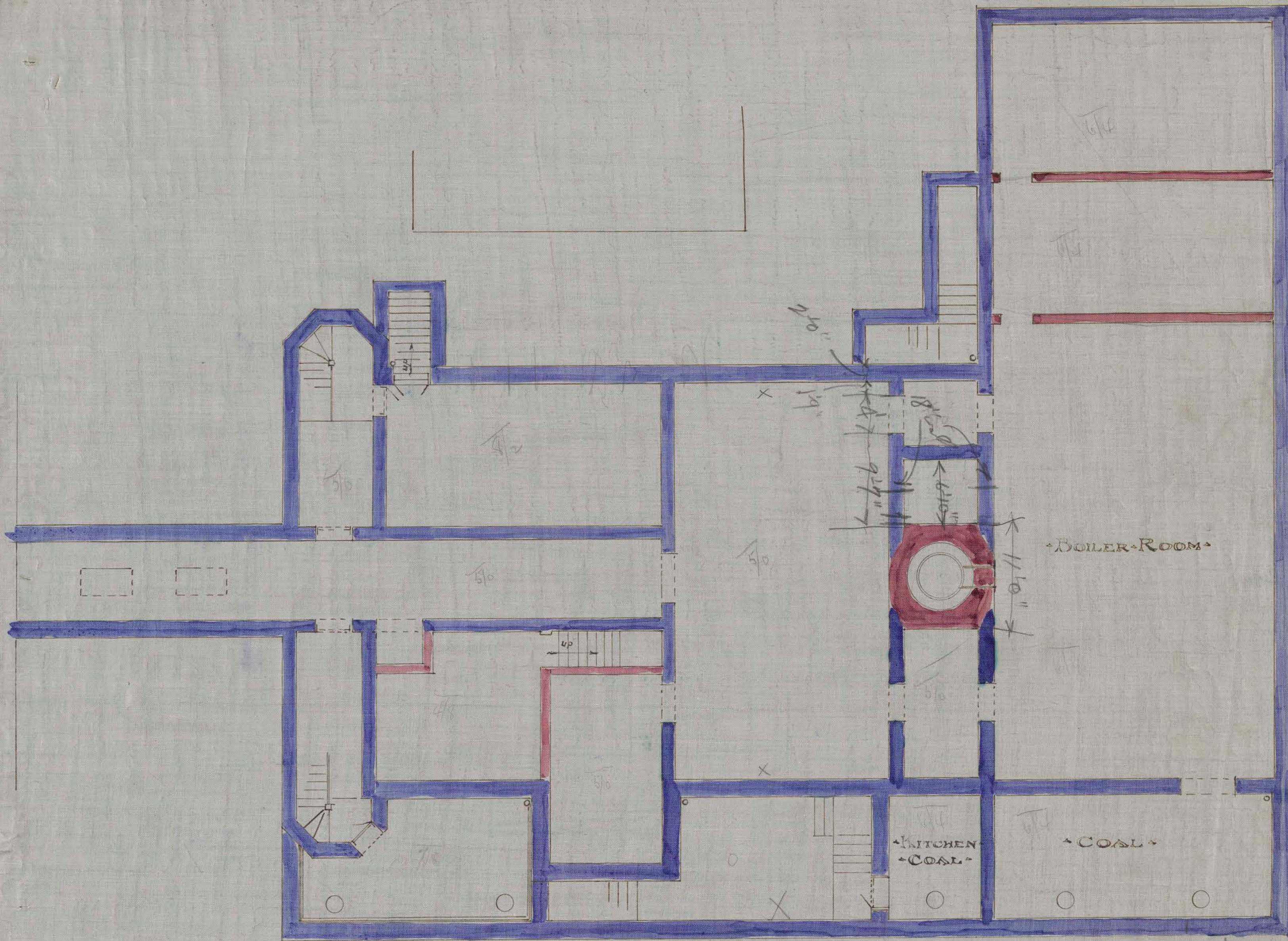
SUB-BASEMENT PLAN SCALE \frac{1}{8}" = 1'
