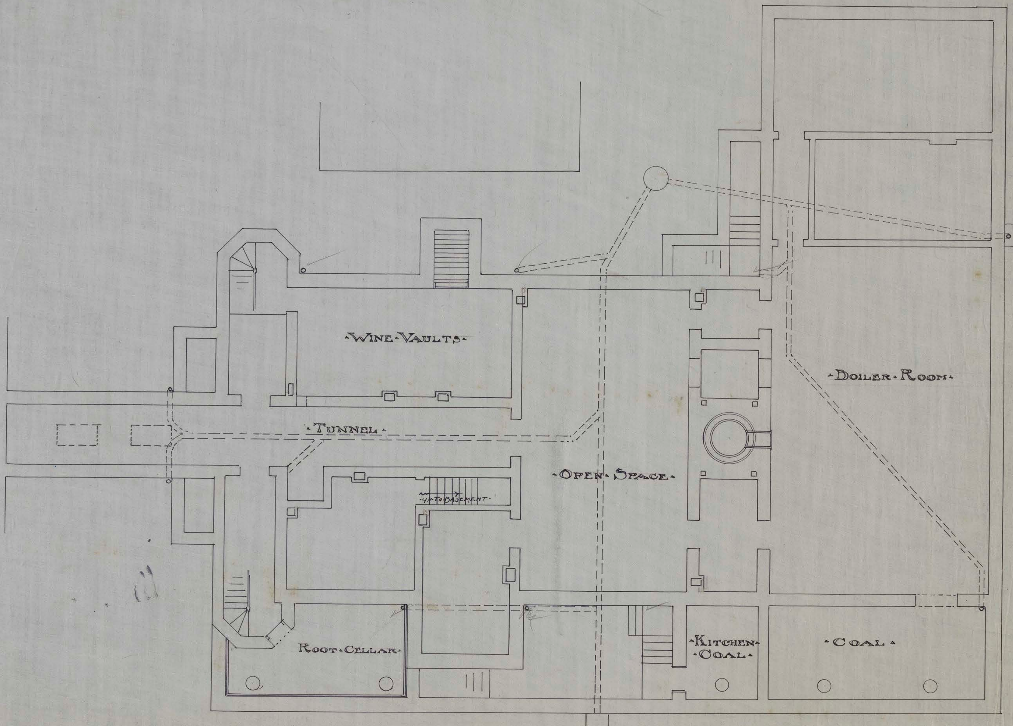
• SUB-BASEMENT PLAN • • SCALE - \frac{1}{8} " •
