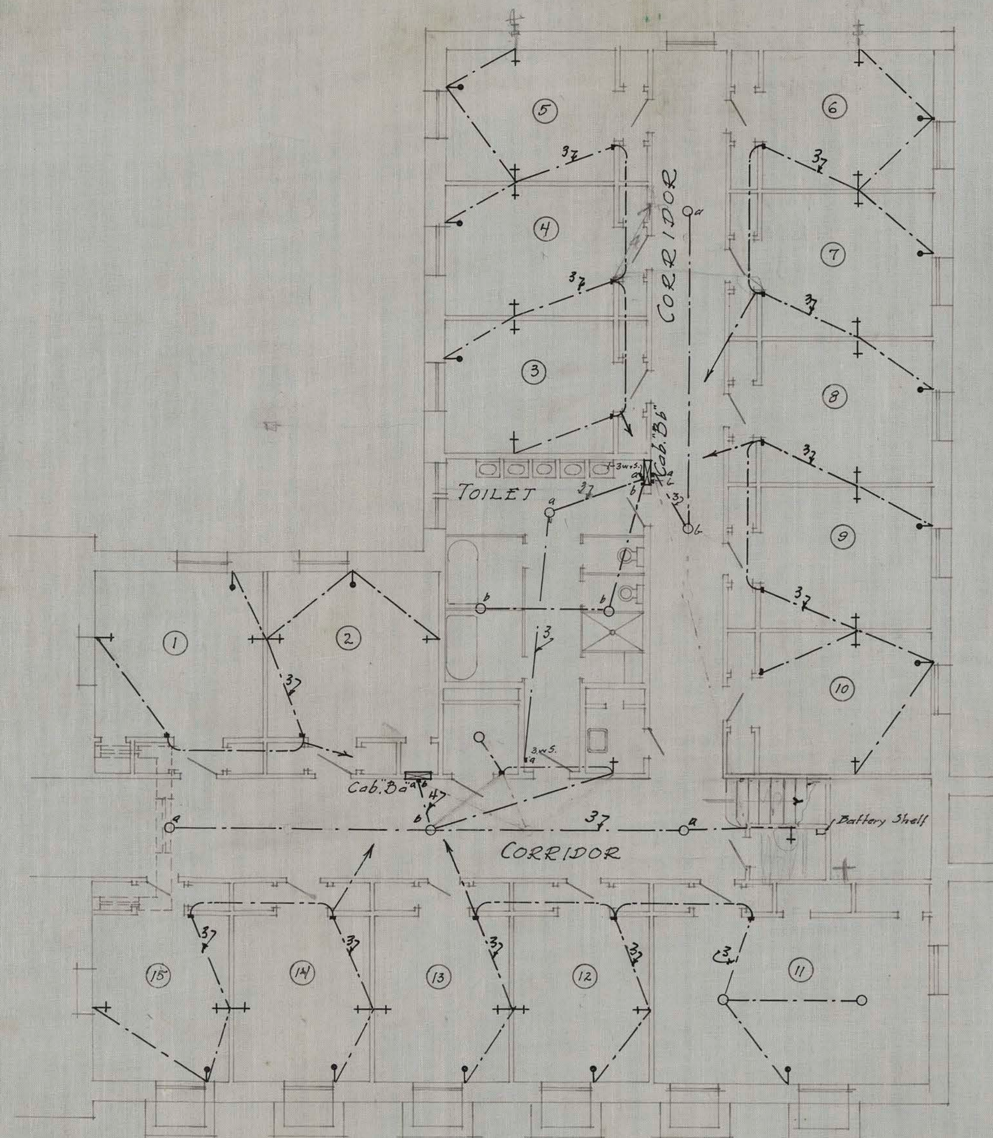
BASEMENT FLOOR PLAN ELECTRICAL
