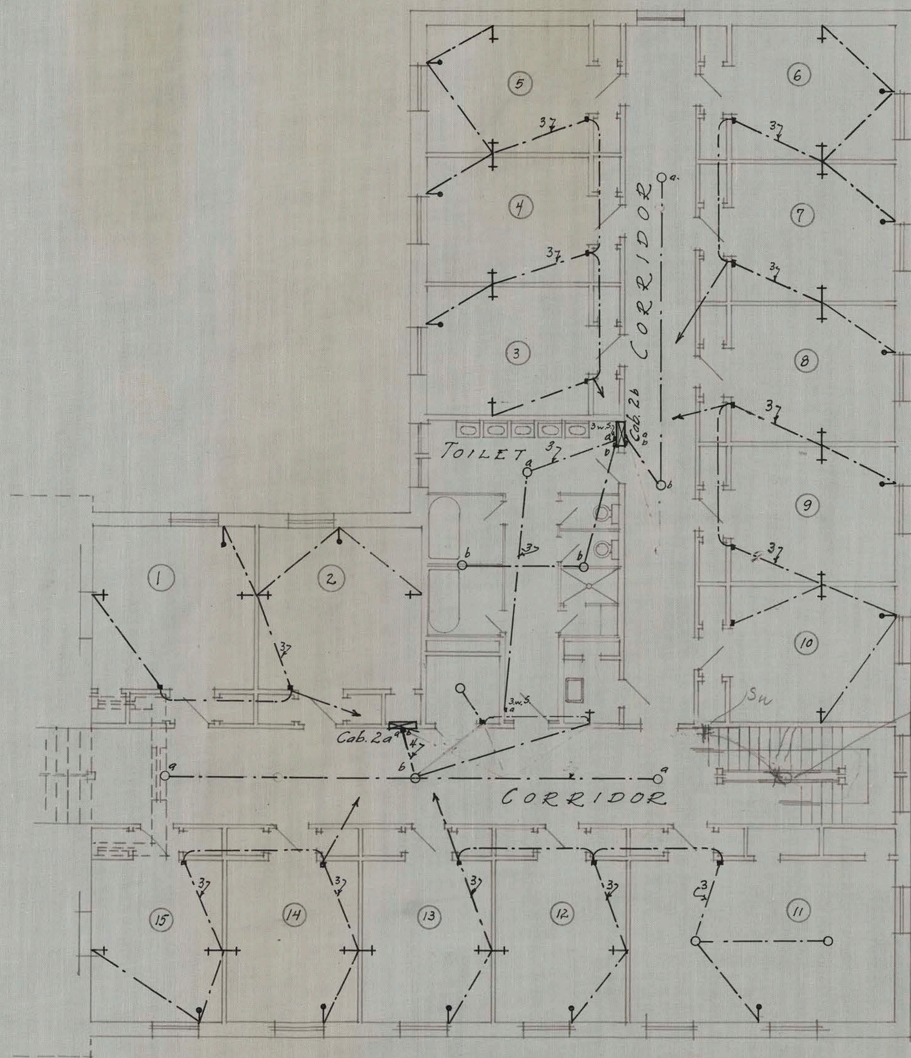
SECOND FLOOR PLAN ELECTRICAL
