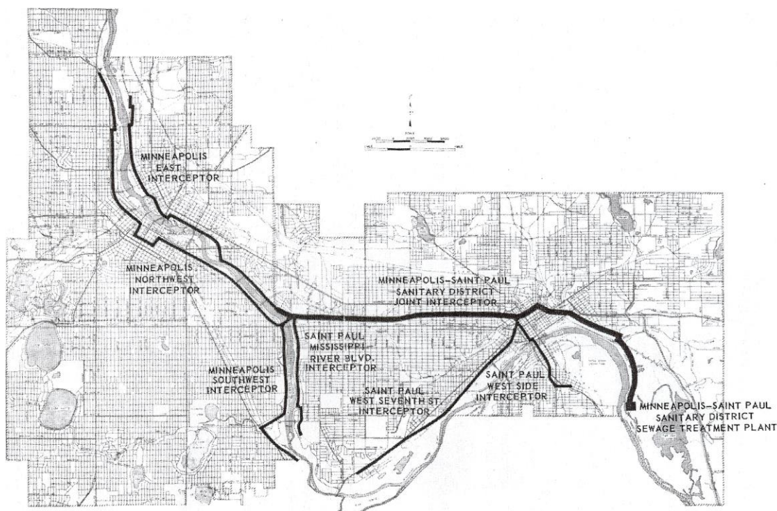
Routes of principal intercepting sewers
