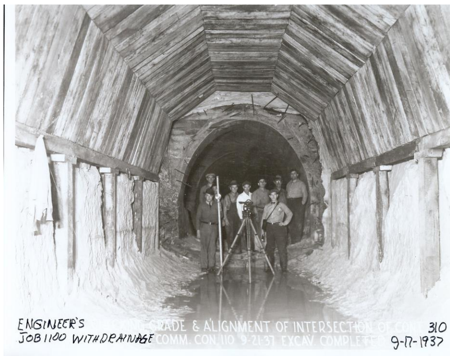
Nine men stand in the St. Peter Sandstone tunnel completed by the City of Minneapolis for a 10'-3" semi-elliptical section sewer that conveys Minneapolis flow from the west side of the Mississippi River from the siphon outlet chamber to the MSSD constructed junction chamber. The location is about 93' below West River Rd north of Marshall Ave in St Paul.
