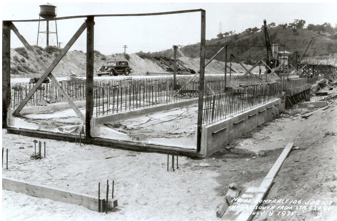
The last section of the Joint Interceptor is a 9'-6" x 10' double barrel sewer which extends about 6000' north from the treatment plant to the bluff shown on the right. The photo shows a section of completed pipe invert, supported by bearing piles. The location is along Childs Rd in St Paul, north of the Metropolitan Treatment Plant, sometimes known as the Pig's Eye Plant, because of its location on Pig's Eye Island.
