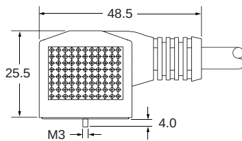
122 Type Connector
