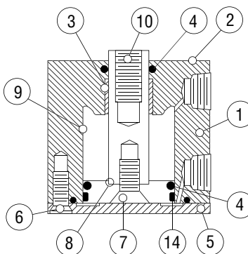
Single Rod – Double Acting Action - X
