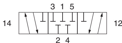
4-Way - 5 Ported - 3 Position - Type B "Blocked"
