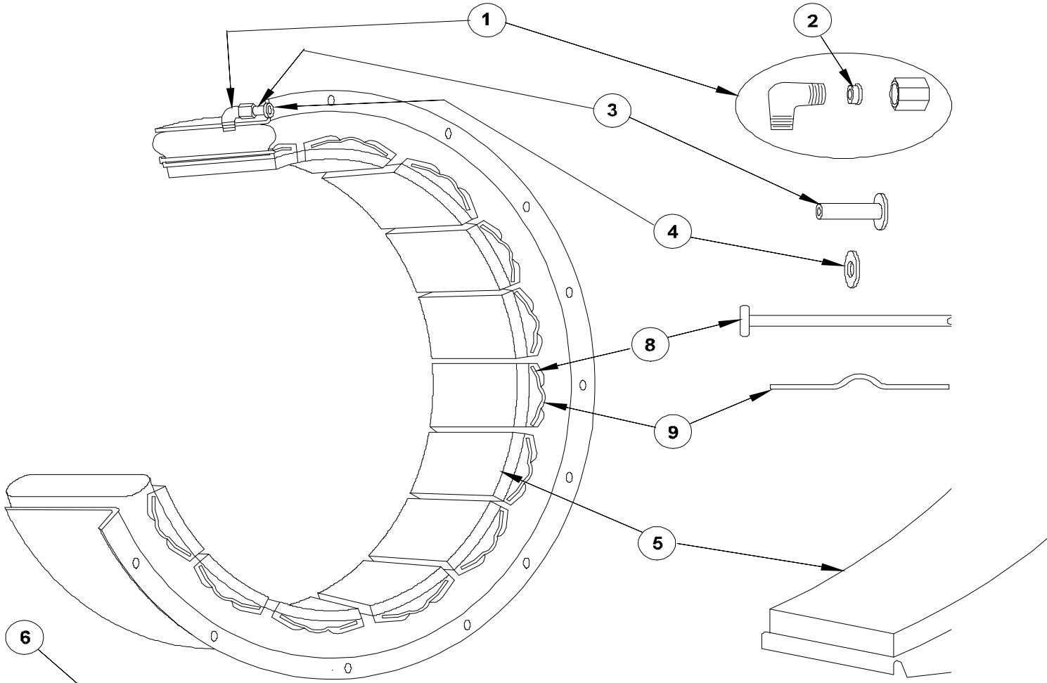
FIG.1 -COMPONENT PARTS FOR AIRFLEX TYPE CB ELEMENT
