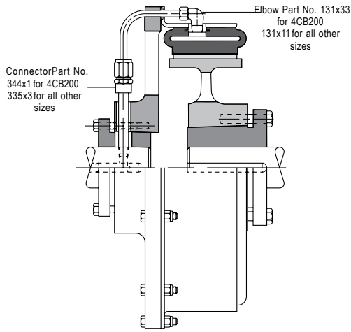
PCB-206 Arrangement
