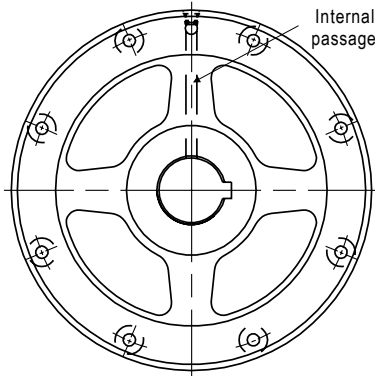
Single Connection
