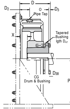
PCB - 208 Arrangement
