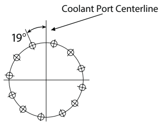
Pressure Plate Coolant Inlet Port 24WCSB 12-0.656 (16,7) Dia. Holes Equally Spaced Holes on a 28.750" (730,3) BC
