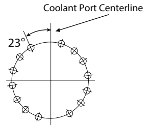
Pressure Plate Coolant Inlet Port 48WCSB 14-1.438 (36,5) Dia. Holes based on 16 Equally Spaced Holes on a 54.000" (1371,6) BC
