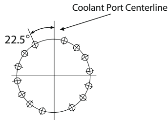
Pressure Plate Coolant Inlet Port 36WCSB 14-1.062 (27,0) Dia. Holes based on 16 Equally Spaced Holes on a 42.000" (1066,8) BC
