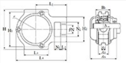
Take-Up Unit, Cast Housing, Adapter, Cast Dust Cover, Closed End, UKT Type - Dimensions
