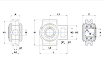
Take-Up Unit, Set Screw, Stainless Steel Housing, One Closed/One Open Cover, SUCT Type - Dimensions
