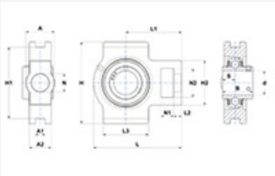
Take-Up Unit, Set Screw, Stainless Steel Housing, SUCT Type - Dimensions
