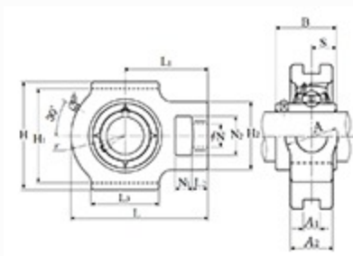
Take-Up Unit, Cast Housing, Set Screw, UCT Type - Dimensions
