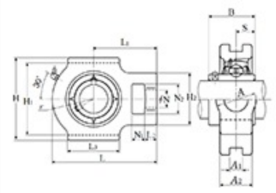
Take-Up Unit, Cast Housing, Set Screw, UCT Type - Dimensions
