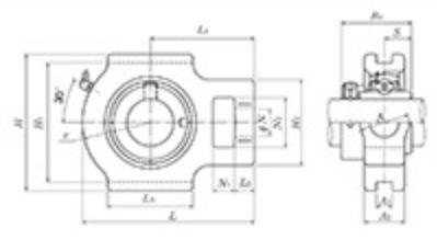
Take-Up Unit, Cast Housing, Eccentric Locking Collar, UELT Type - Dimensions
