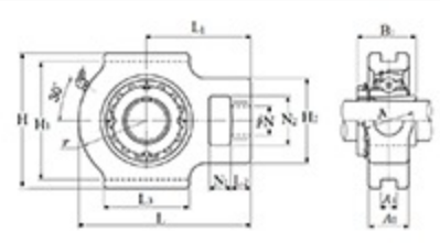
Take-Up Unit, Cast Housing, Adapter, UKT Type - Dimensions
