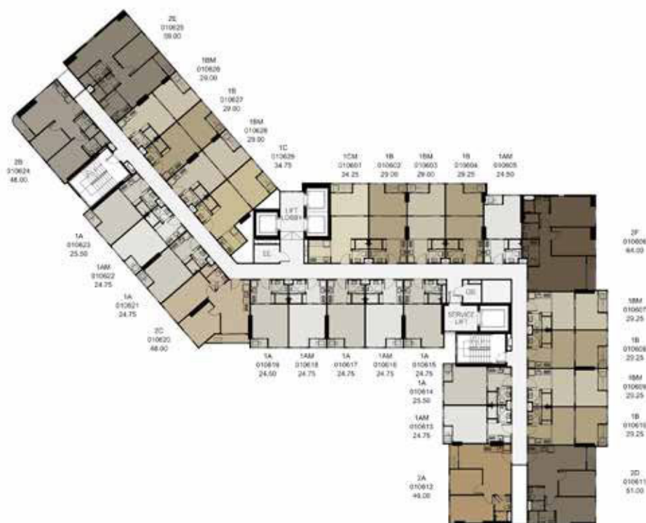
6 th - 19 th FLOOR PLAN
