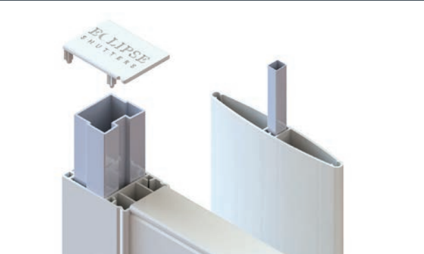
ALUMINUM REINFORCEMENT
